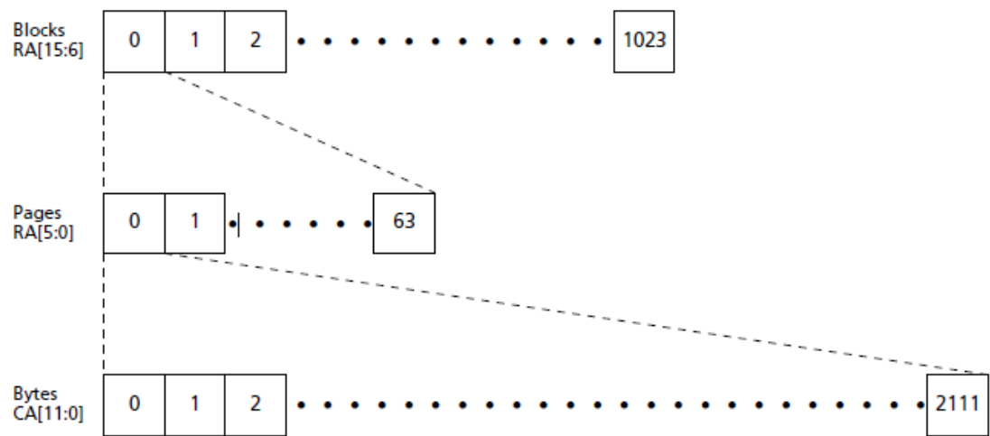
Figure 1.3 Address Map
