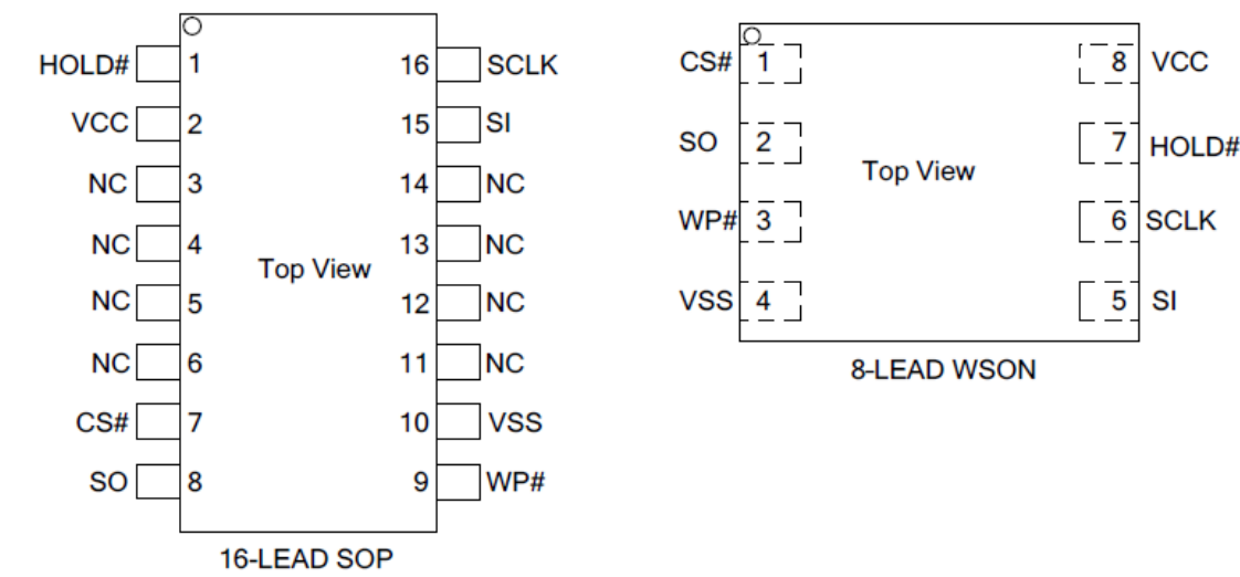
Figure 6.1 Pin Configuration
